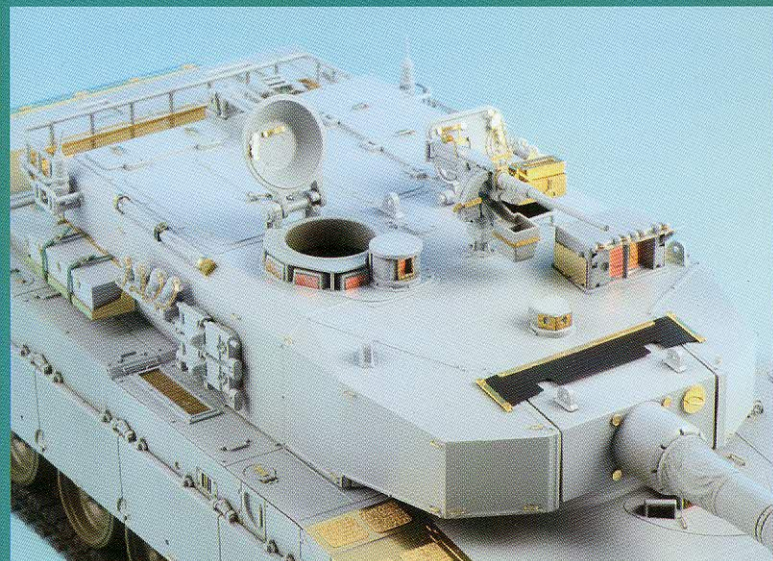
1/35 JGSDF TYPE90 (for TAMIYA)
