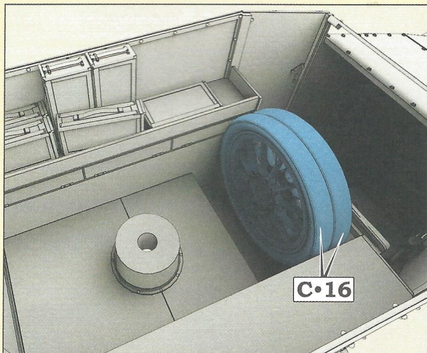
Step 49. Installing the spare wheels
