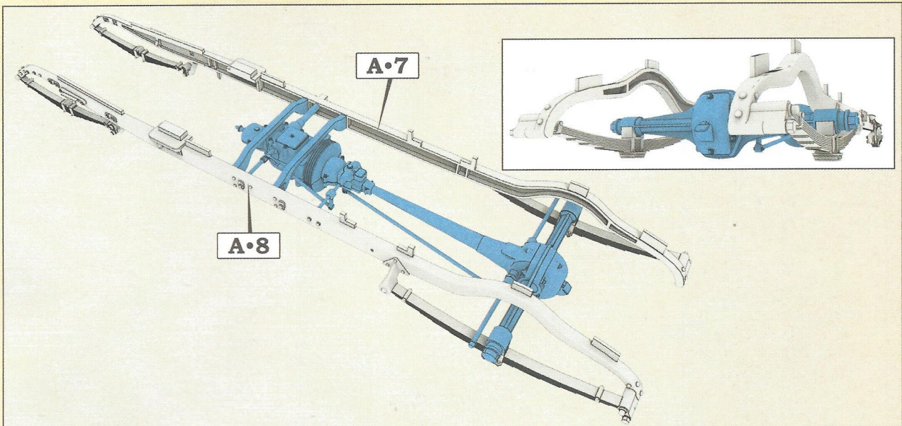
Step 6. Installing both side rails
