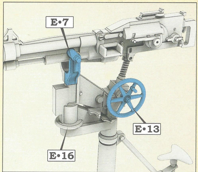
Step 46. Assembling the Saint-Étienne MG mount
