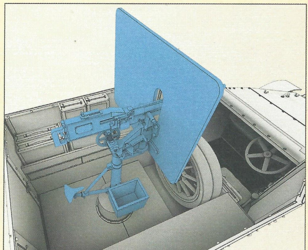
Step 50. Installing the MG into the car
