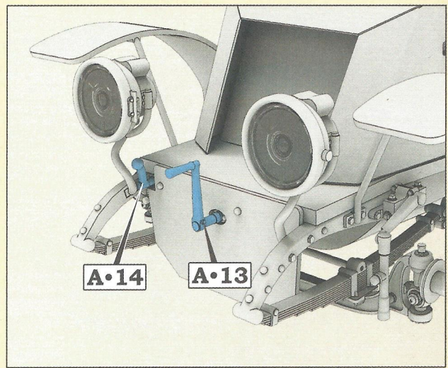
Step 37. Installing the lever and hand crank
