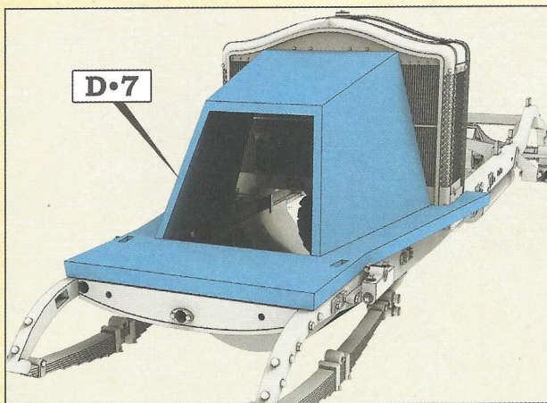
Step 14. Installing the engine protection
