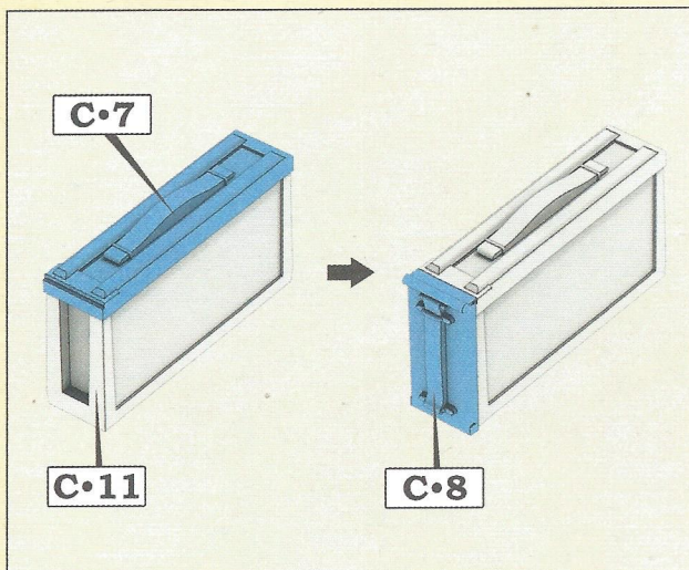
Step 43. Assembling the ammunition boxes. Make six
