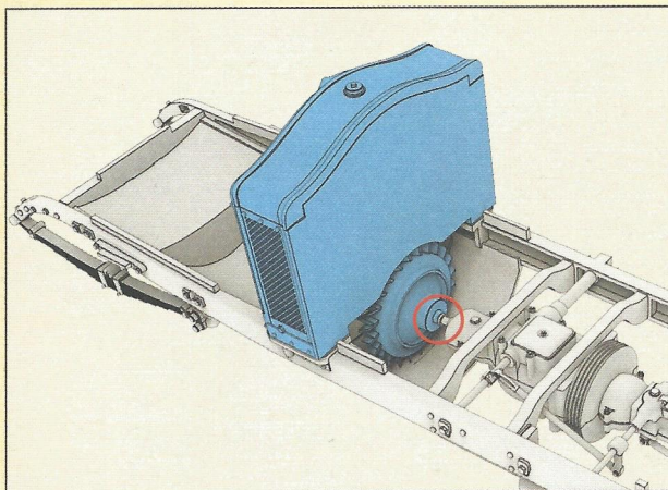
Step 12. Installing the radiator
