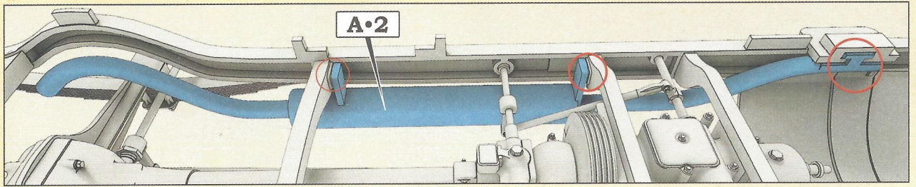
Step 10. Installation of the exhaust pipe with muffler
