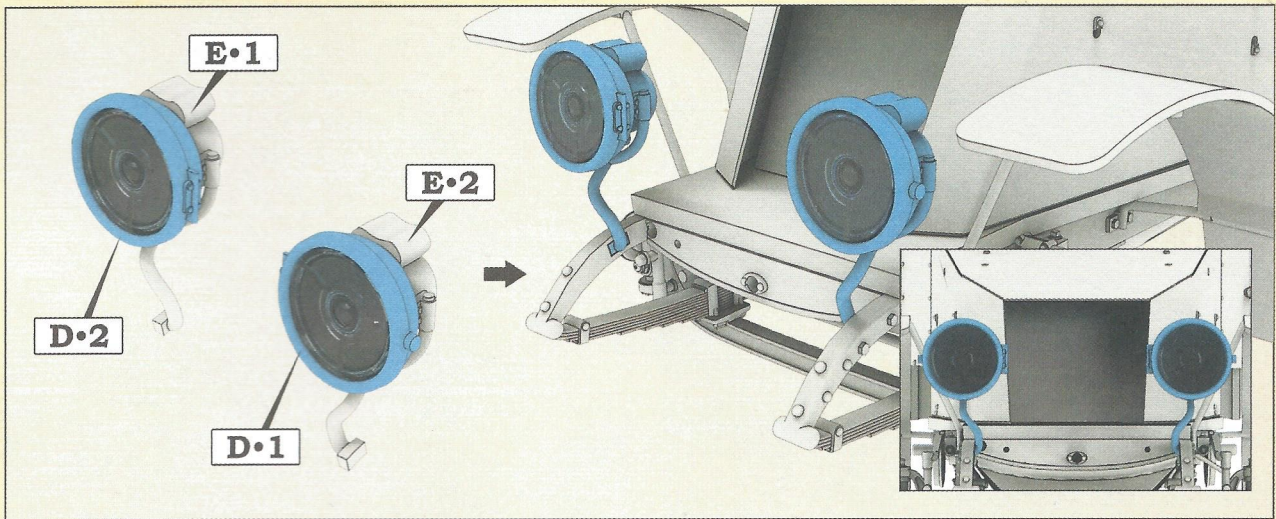
Step 35. Assembling and installing the headlights
