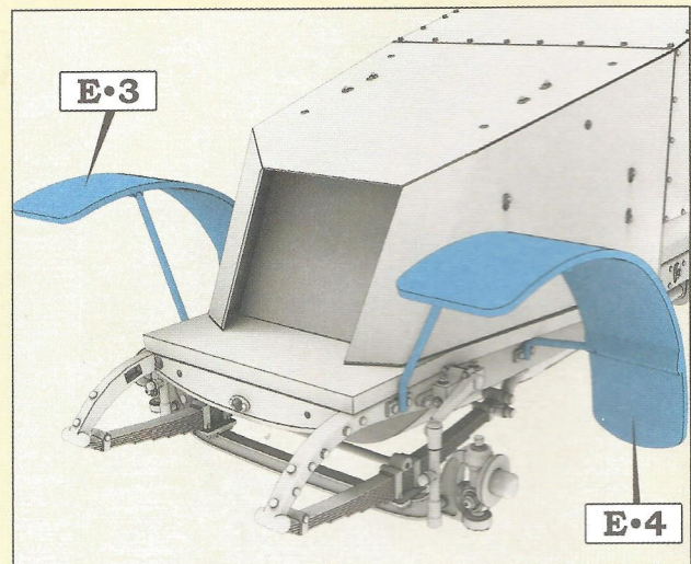
Step 34. Installation of the front fenders
