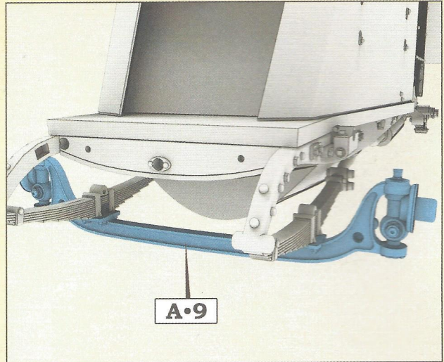
Step 30. Installation of the front axle
