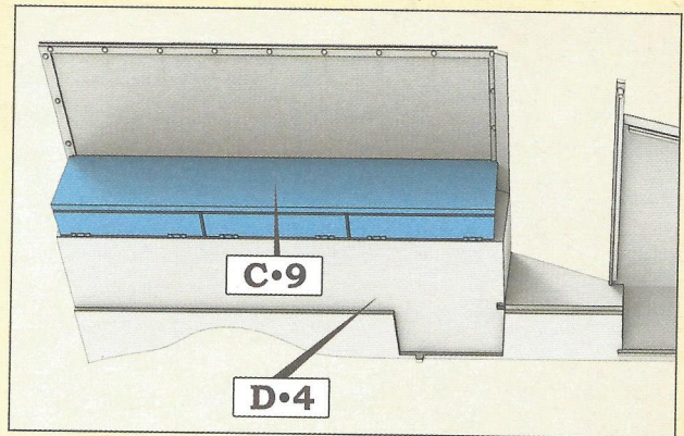
Step 17. Installing the port stowage boxes
