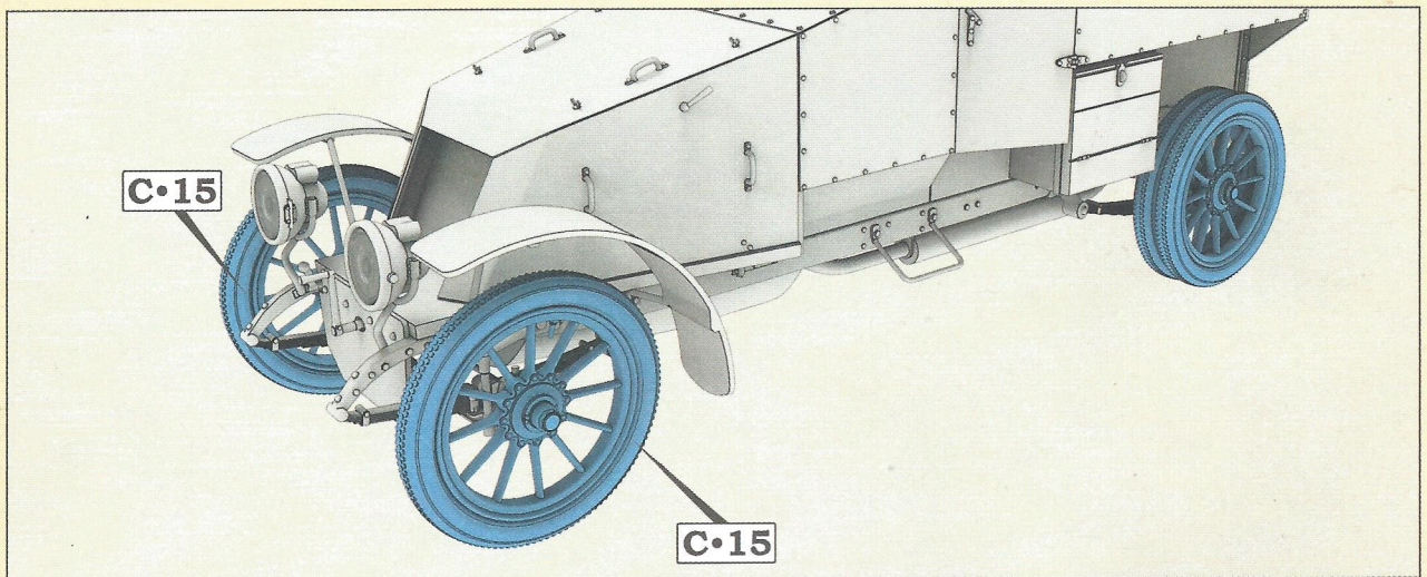
Step 42. Installation of the front and rear wheels
