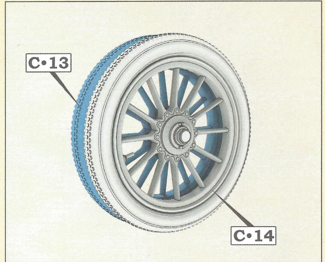
Step 41. Assembling the rear twin-wheel
