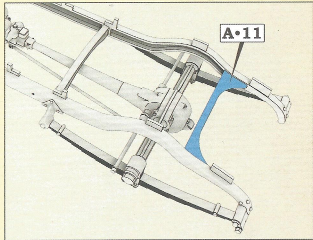
Step 8. Installing the rear cross member
