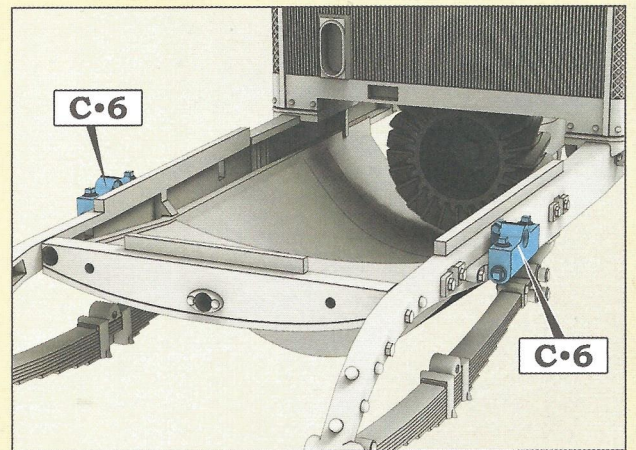
Step 13. Shock absorber blocks installation
