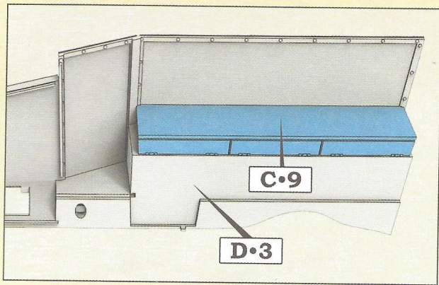
Step 16. Installing the starboard stowage boxes
