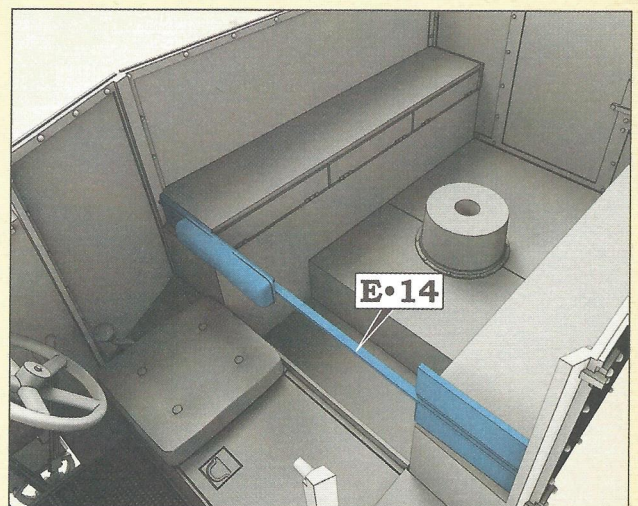
Step 26. Installing the driver's backrest with the compartment cross member
