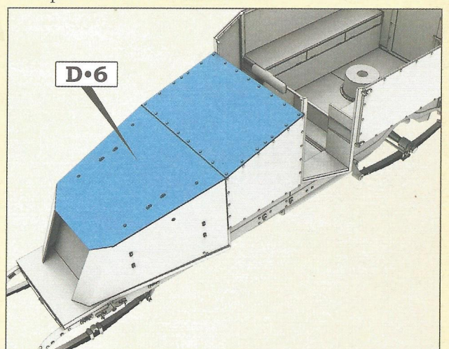
Step 28. Installing the engine hood
