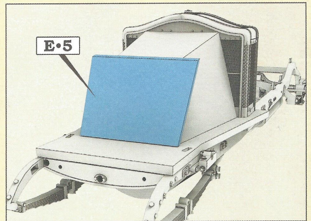
Step 15. Installation of the front engine armour plate
