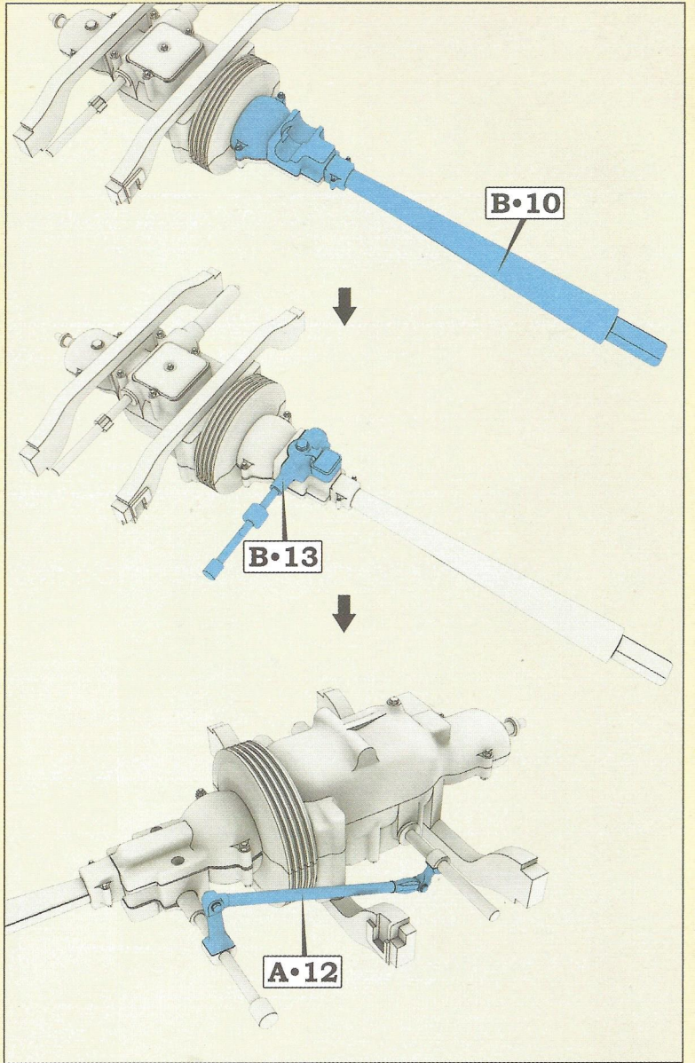
Step 3. Installing the drive shaft
