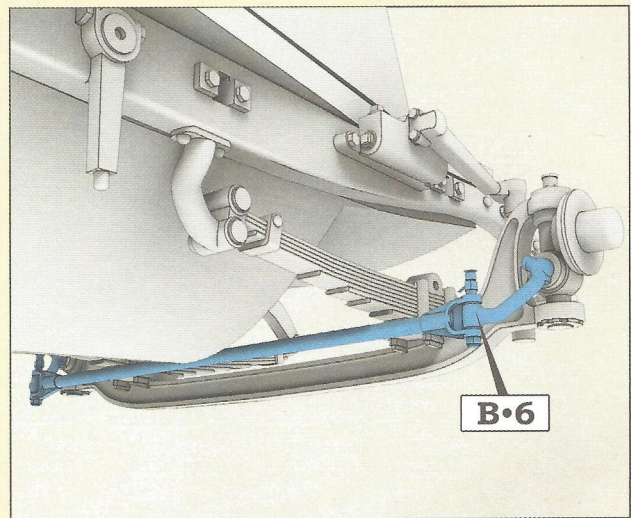
Step 32. Installing the track-rod
