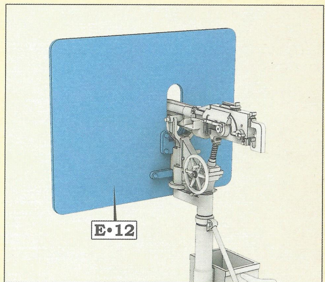
Step 48. Installing the MG shield. Not for all markings
