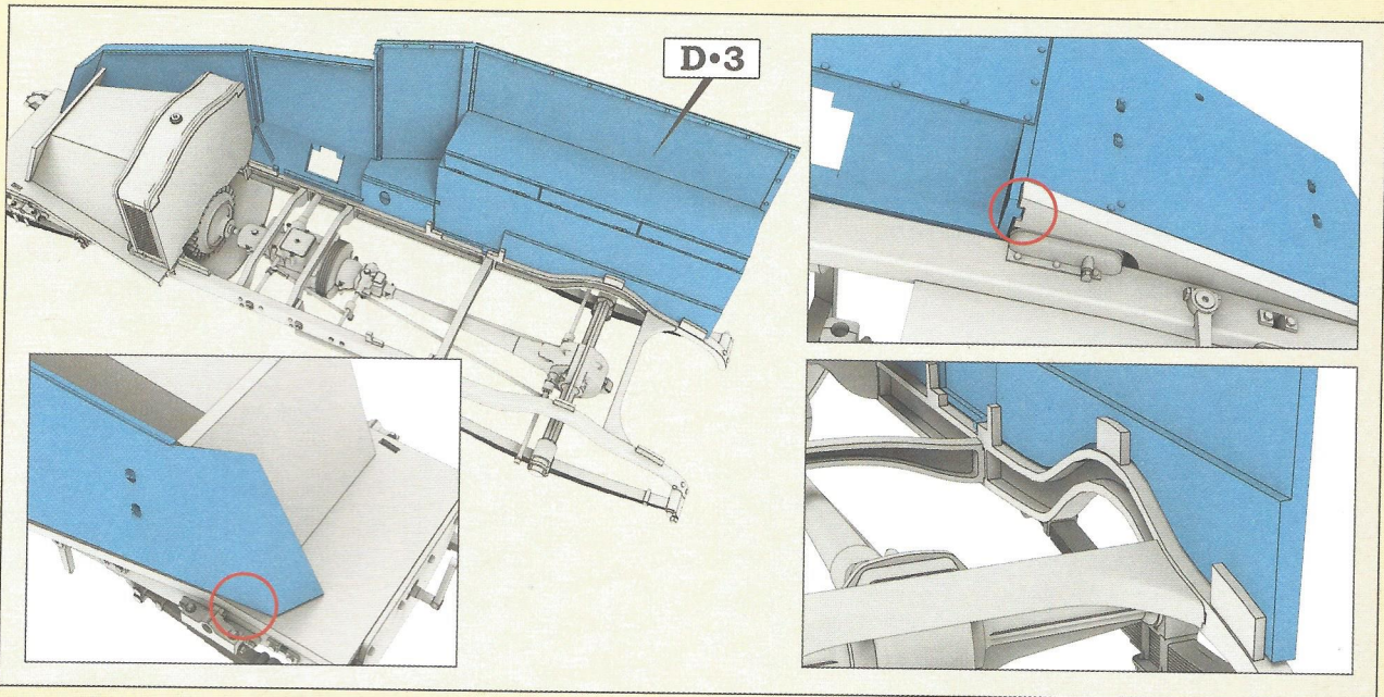
Step 18. Installation of the starboard armoured superstructure wall
