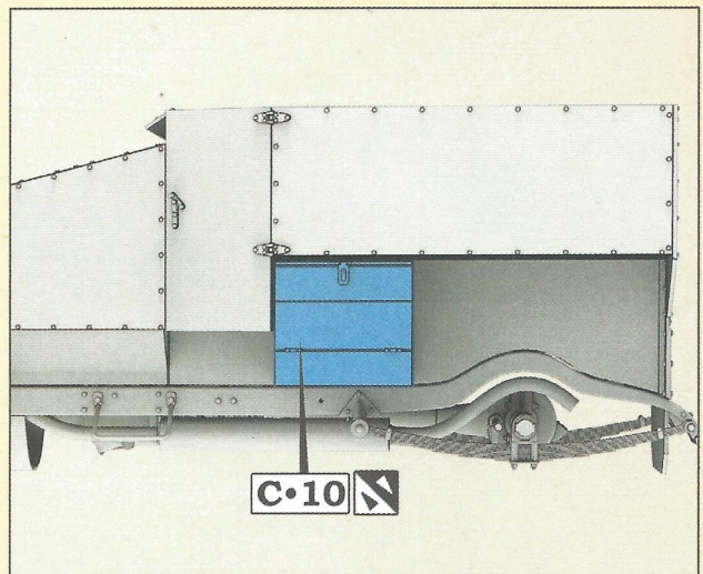
Step 39. Installation of the outside stowage boxes. On both sides of the car
