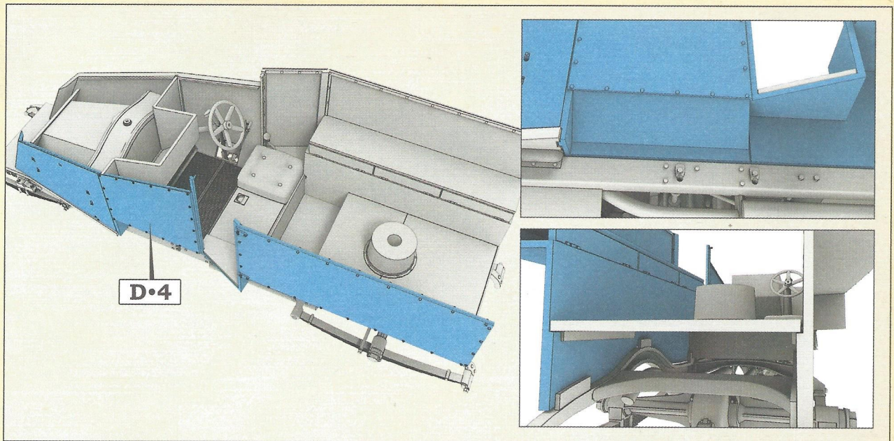
Step 24. Installation of the port armoured superstructure wall
