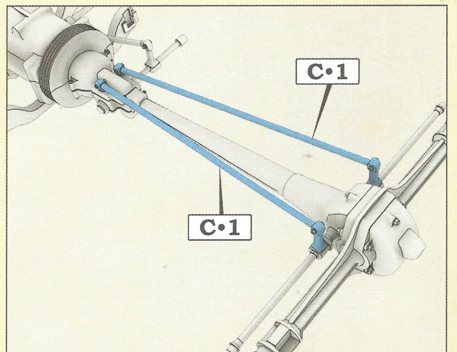
Step 5. Installing the rear radius rods
