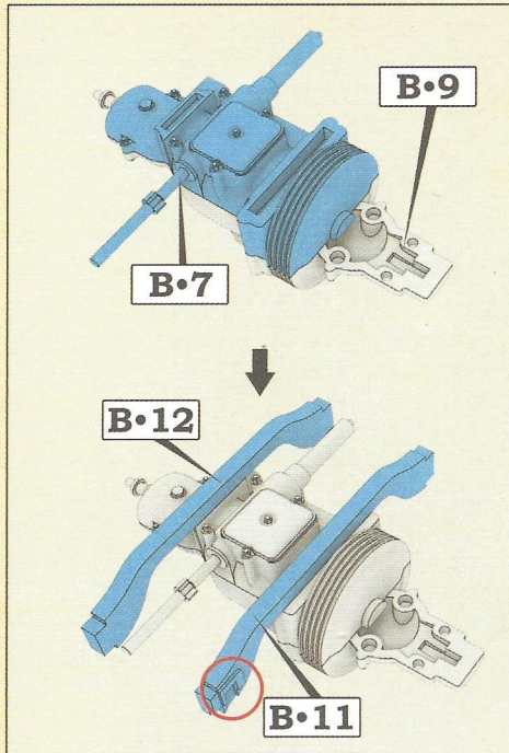
Step 1. Assembling the gearbox
