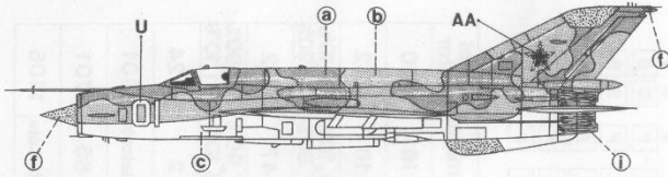
1 MiG-21bis-SAU Fishbed N, Soviet Air Force, 1989.
