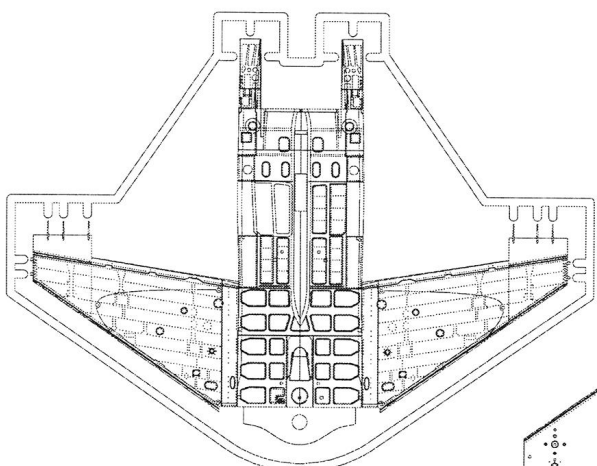
Upper fuselage
