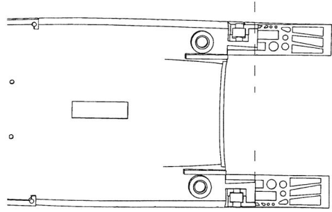
Upper Fuselage
