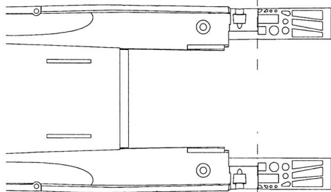
Lower Fuselage
