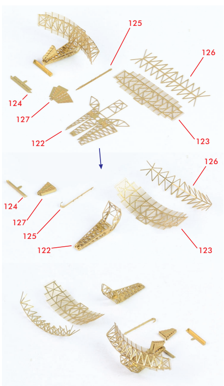
<AN/SPS-49 RADAR>
