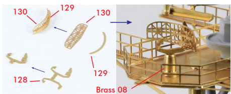
<AN/SPS-49 RADAR>
