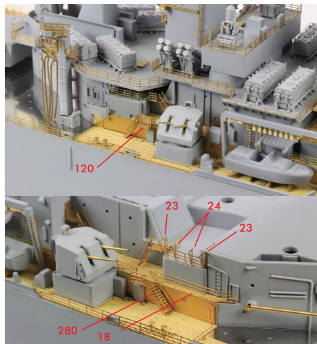
<Ladder ETC.>
