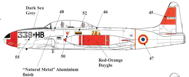
T-33A CEVSV, Toul, early 1970's. (Ref: Loose file - Ler Fanu DAVIATION P.12).
