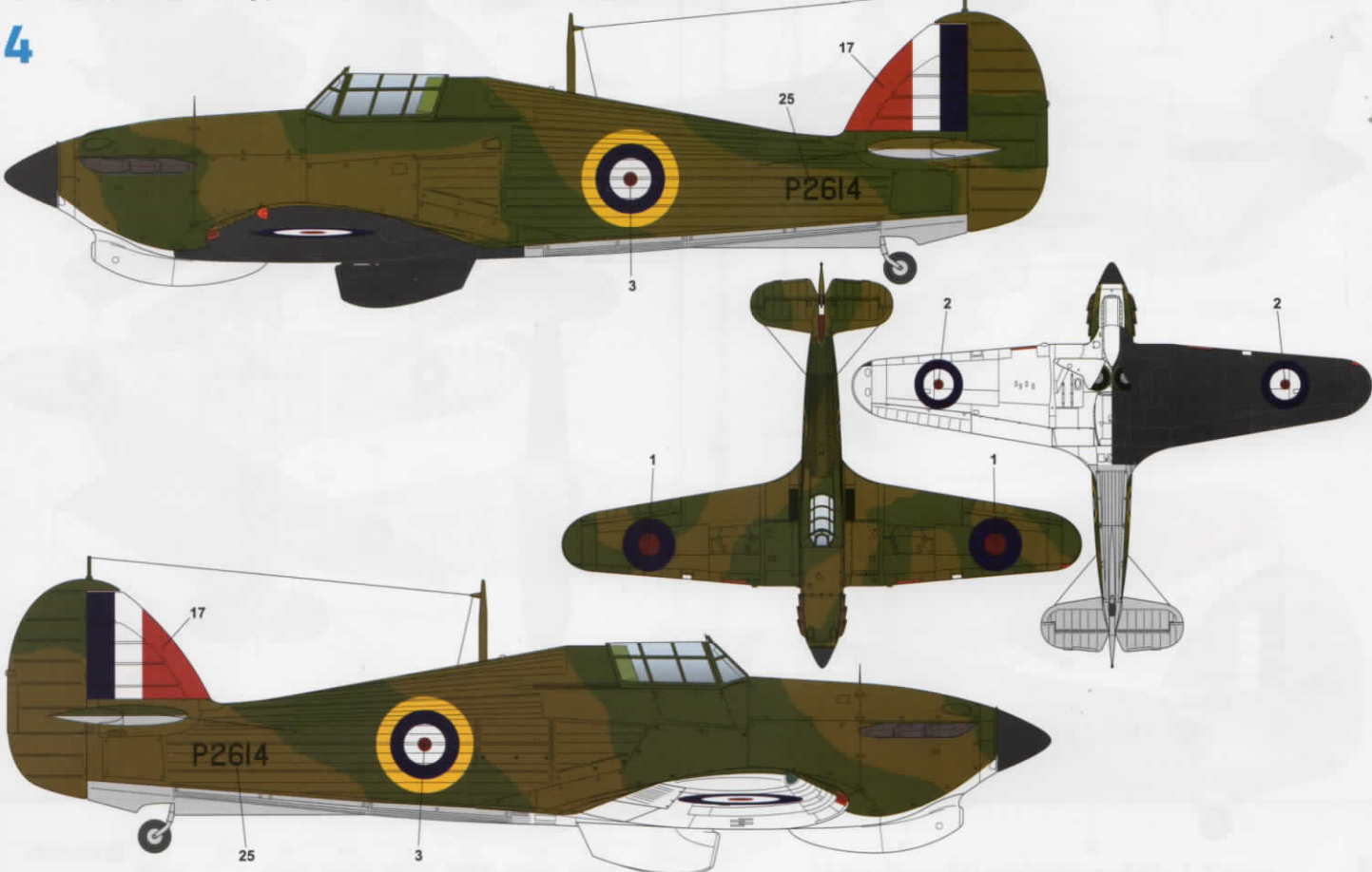
Hurricane Mk.I Trop, one of five Hurricanes delivered to Malta in June 1940
