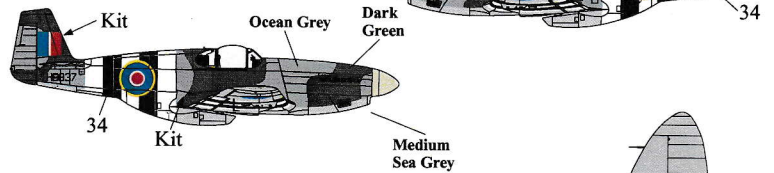
North American Mustang III, HB837 of No.617 Squadron, flown by Wg.Cdr. Leonard Cheshire, DSO,DFC, from RAF Woodhall Spa, July/August 1944.
