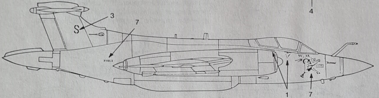
BUCCANEER S2B XV863/S "Debbie-Sea Witch"
